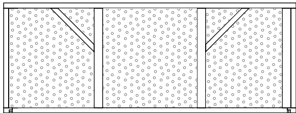
Spa frame with foam inserted
