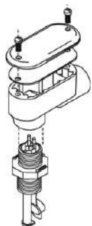
6000-540 , Flow switch only
