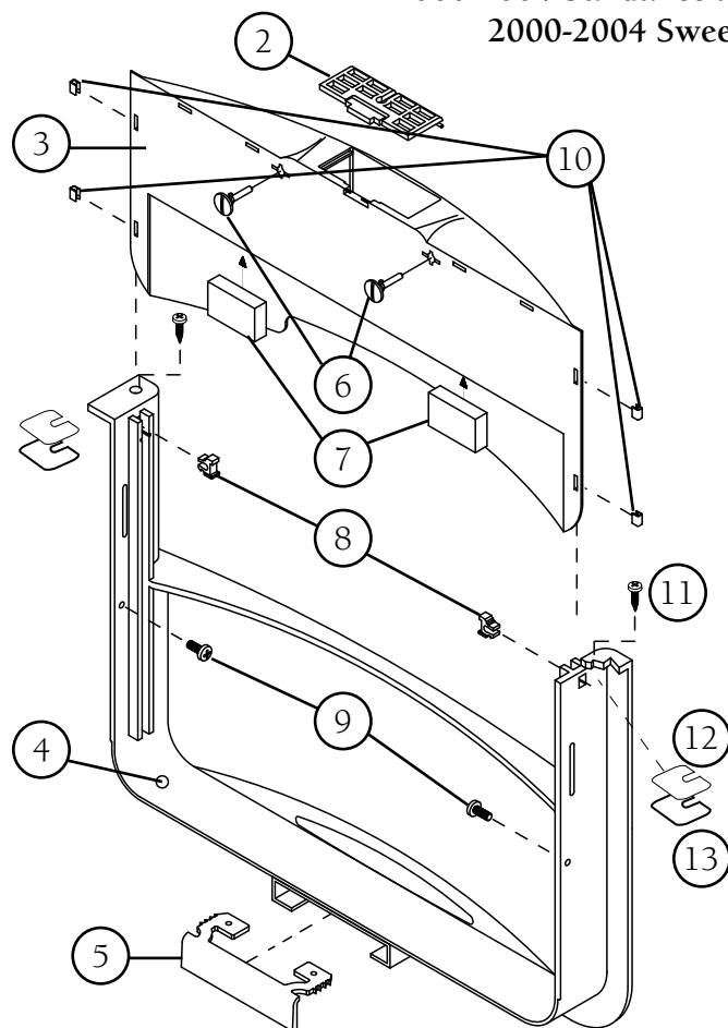
Weir Assembly (Back)
